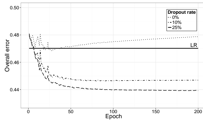
Figure 5: The overall error decreasing curves of D-GEX-9000 \times 2 on GTEx-te with different dropout rates. The x-axis is the training epoch and the y-axis is the overall error. The overall error of LR is also included for comparison.
