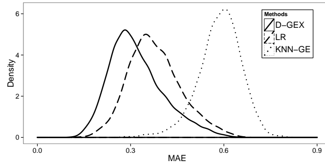
Figure 2: The density plots of the predictive errors of all the target genes by LR, KNN-GE and GEX-10%-9000 \times 3 on GEO-te.
